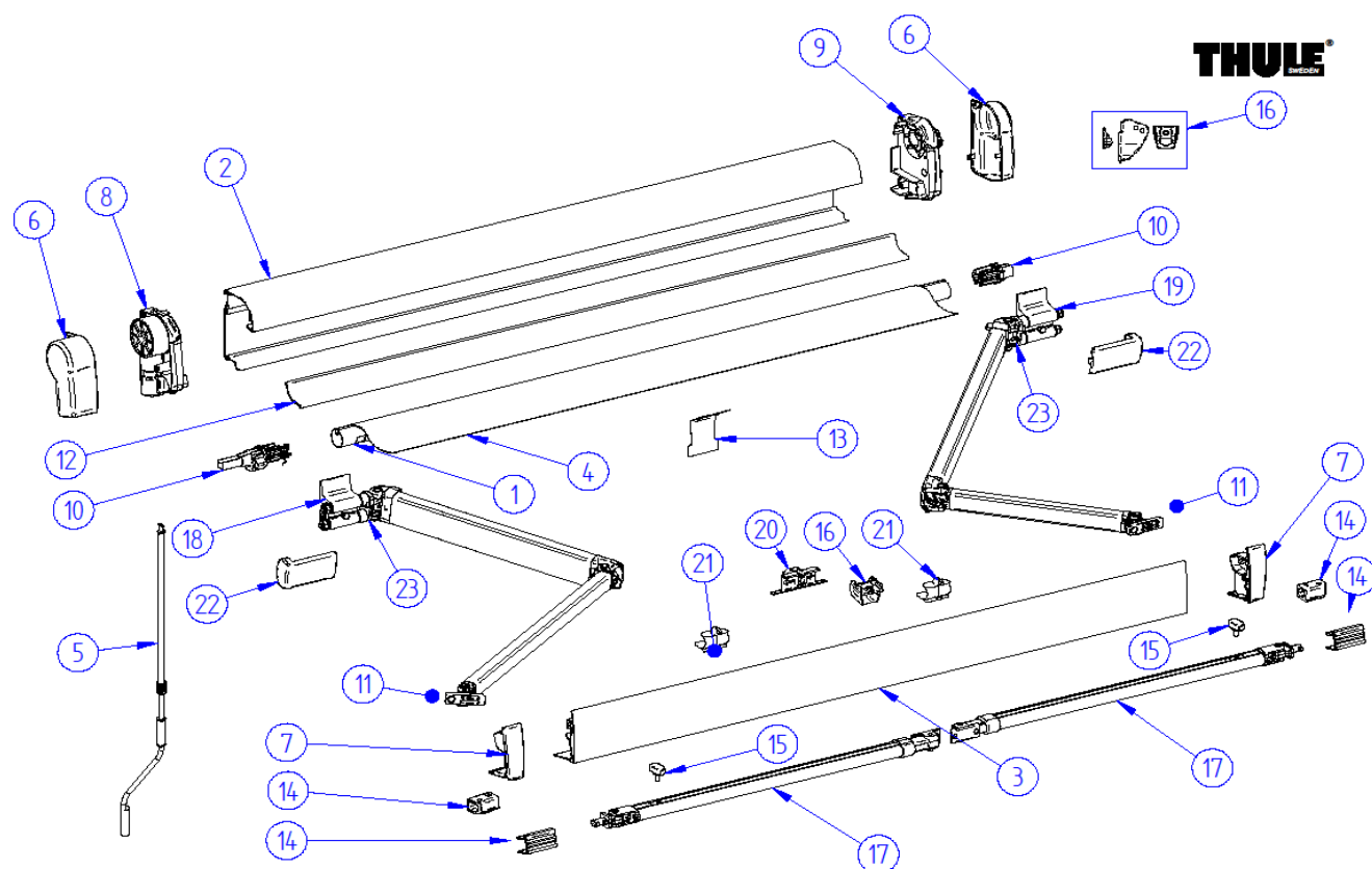
THULE Omnistor 4900 & Tristor 2
