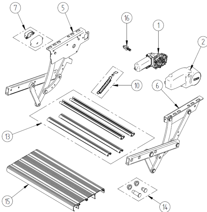
THULE Single step V15 12V & Manual
