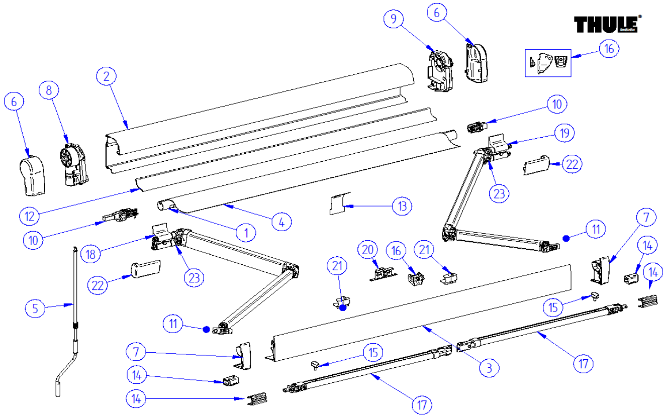
THULE Omnistor 4900 & Tristor 2
