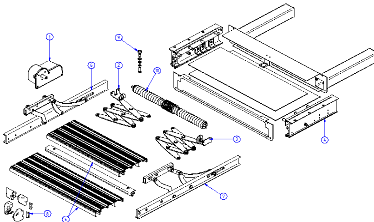
THULE Slide out 600
